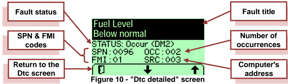
Figure 10 - "Dtc detailed" screen
